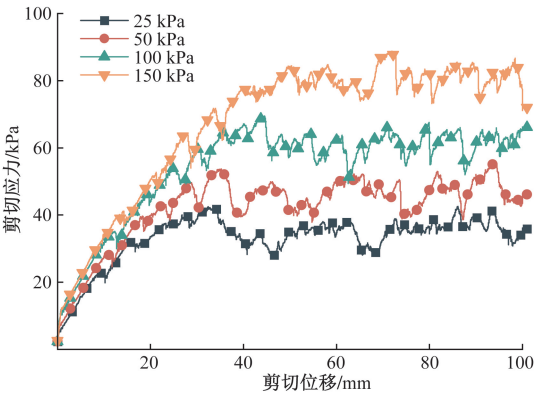
图 9 横肋高度为 100 mm 的土工织物剪应力-位移关系曲线 Fig. 9 Shear stress-displacement relationship curve of geotextile with 100 mm transverse rib height
